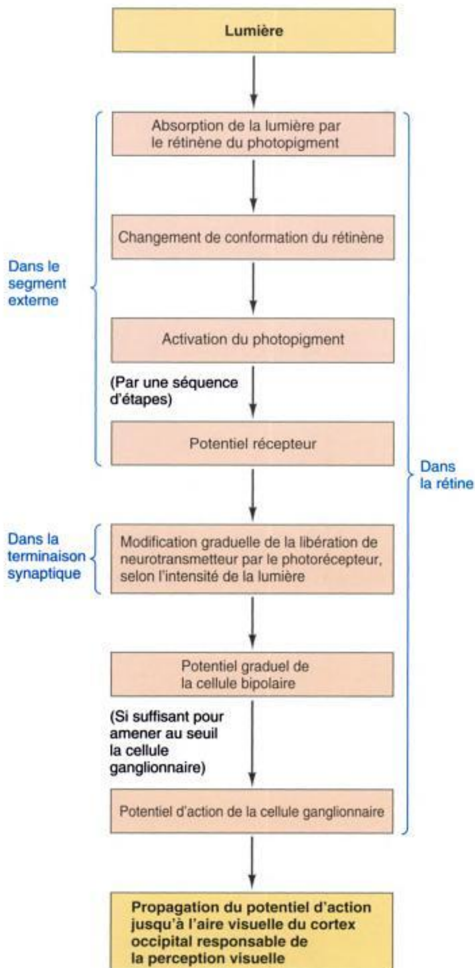
● FIGURE 6-21 Phototransduction
