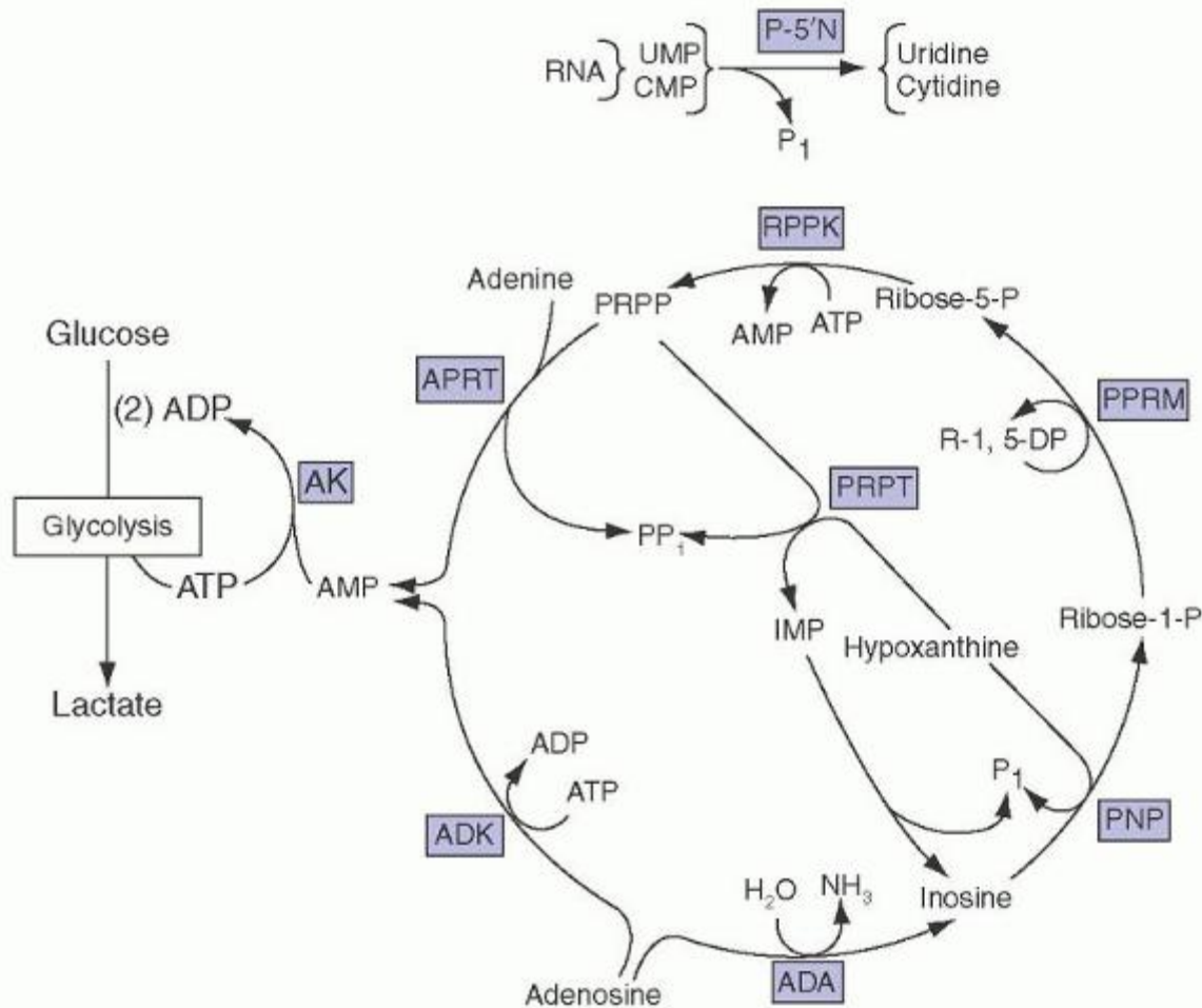
FIGURE 28.5. Schema of purine and pyrimidine metabolism in mature erythrocytes. Enzyme abbreviations: ADA, adenosine deaminase; ADK, adenosine kinase; AK, adenylate kinase; APRT, adenine phosphoribosyltransferase; RPPK, ribopyrophosphoryl kinase; PPRM, pyrophosphoribosyl mutase; PPRT, pyrophosphoribosyl transferase; PNP, purine nucleoside phosphorylase; P5'N pyrimidine 5' nucleotidase. Substrate abbreviations: AMP, adenosine monophosphate; IMP, inosine monophosphate.
