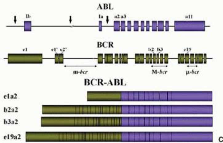
FIGURE 81.1. A: Metaphase karyogram of a newly diagnosed man with CML. The yellow arrows indicate the derivative chromosome 9 and the Philadelphia chromosome (Ph). B: Schematic of chromosomes 9, 22 and the derivatives resulting
