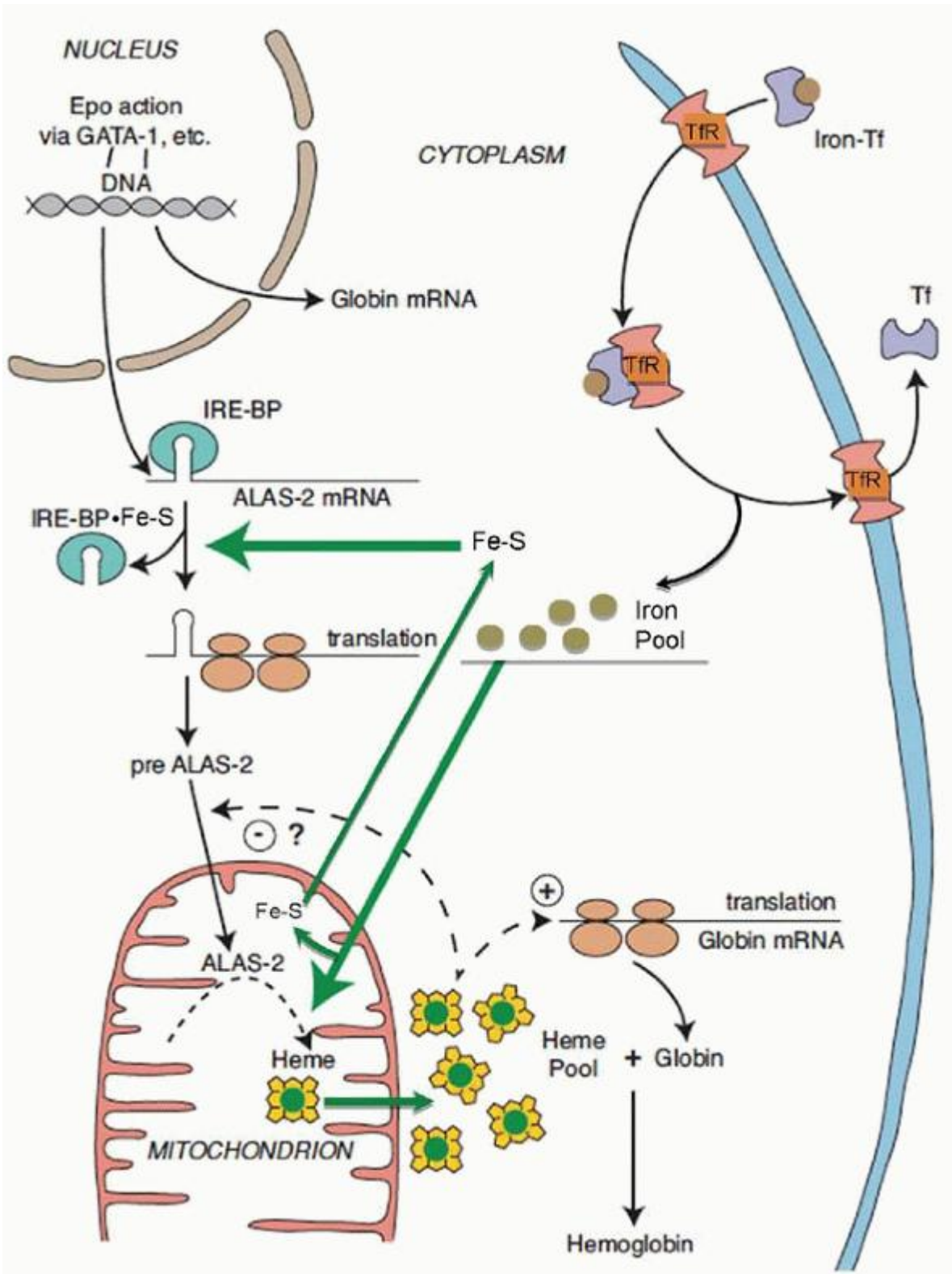
FIGURE 24.2. Pathways of regulation of erythroid 5-aminolevulinate synthase (ALAS2). Epo, erythropoietin; Fe-S, iron-sulfur cluster; Tf, transferrin; TfR, transferrin receptor; IRE-BP, iron-responsive element binding protein; - denotes inhibition, + denotes stimulation. (Modified from May BK, Dogra SC, Sadlon TJ, et al. Molecular regulation of heme biosynthesis in higher vertebrates. Progr Nucleic Acid Res Mol Biol 1995;51:1-51.)
