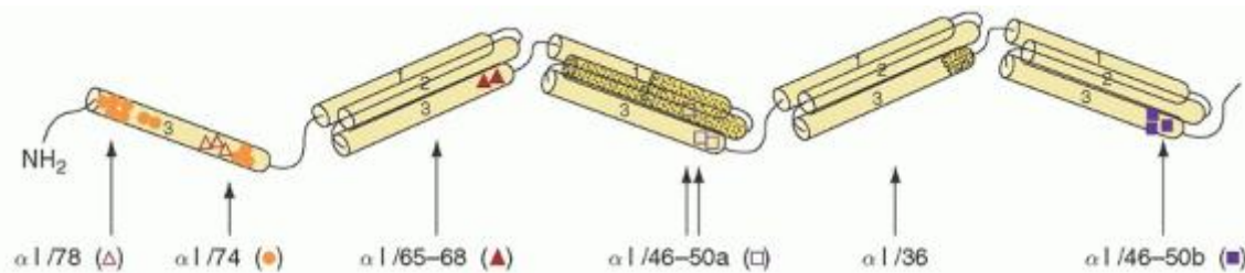
FIGURE 27.10. Defects of the \alpha\beta -spectrin self-association site in hereditary elliptocytosis (HE) and hereditary pyropoikilocytosis (HPP). A model of the triple helical spectrin repeats that constitute the \alpha\beta -spectrin self-association site is shown. Limited tryptic digestion of spectrin, followed by two-dimensional gel electrophoresis, identifies abnormal cleavage sites (arrows) in spectrin associated with various mutations. Symbols denote positions of various genetic defects identified in patients with HE or HPP. In most cases, the mutation found is adjacent to the abnormal cleavage site, either in the same helical coil or in helical coils juxtaposed next to each other in the triple helical model. The hashed lines denote the location of spectrin chain truncations. (Reprinted and modified with permission from Gallagher PG, Tse WT, Forget BG. Clinical and molecular aspects of disorders of the erythrocyte membrane skeleton. Semin Perinatol 14:351,1990.)
