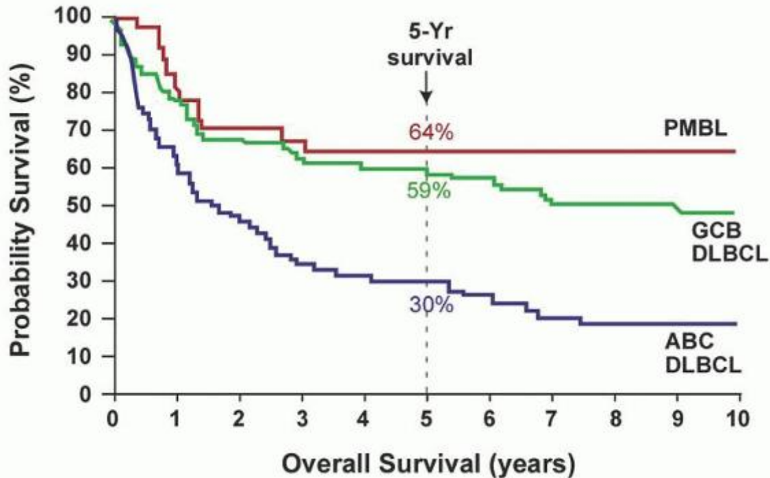
FIGURE 88.14. Gene expression arrays can stratify diffuse large B cell lymphoma (DLBCL) into at least three subtypes, primary mediastinal B cell lymphoma (PMBL), germinal center B cell (GCB), and activated B cell-like (ABC). This Kaplan-Meier curve indicates differing survival among the groups. From Rosenwald A, Wright G, Leroy K, et al. Molecular diagnosis of primary mediastinal B cell lymphoma identifies a clinically favorable subgroup of diffuse large B cell lymphoma related to Hodgkin lymphoma. J Exp Med 2003;198:851-862, with permission.
