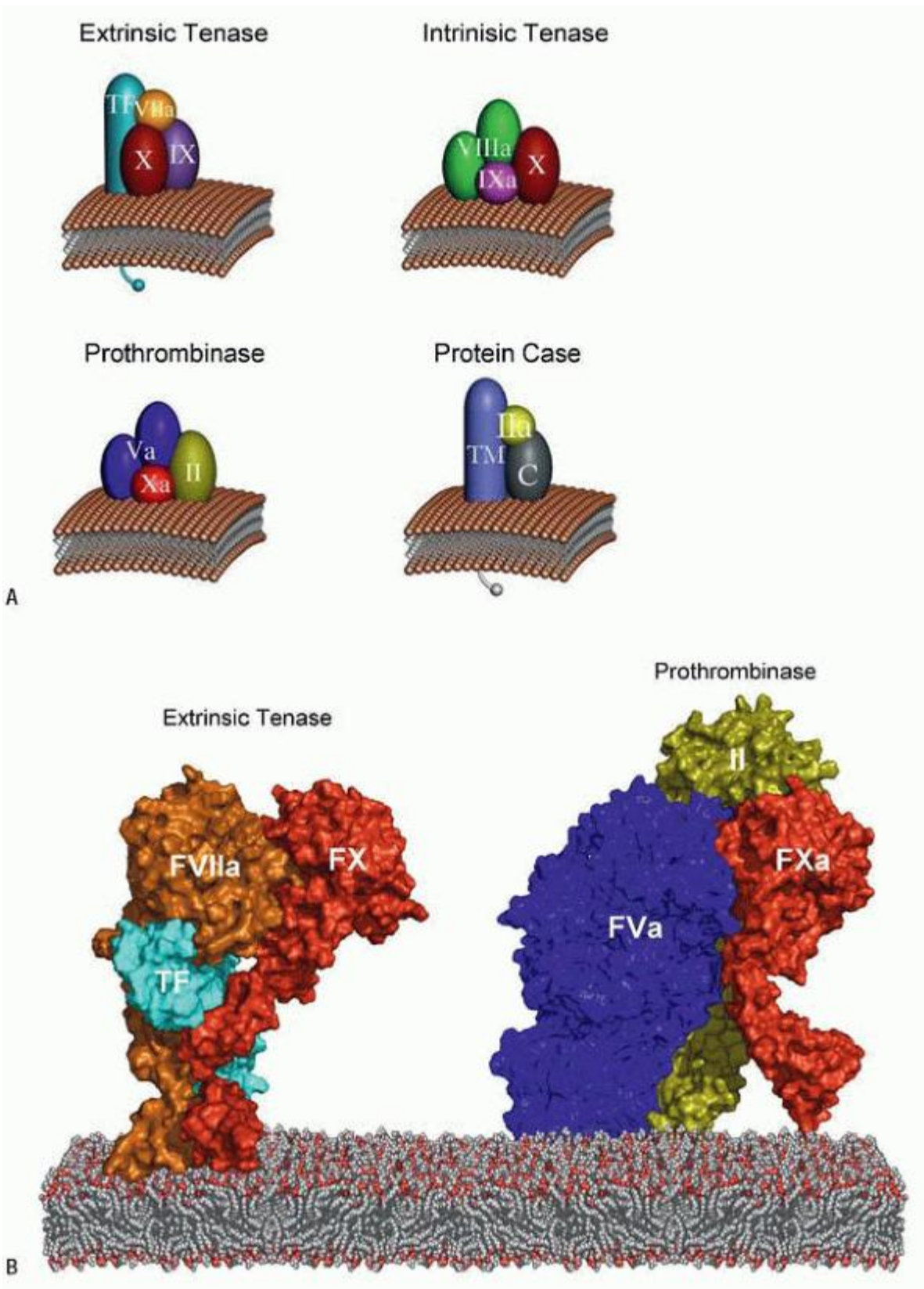
FIGURE 18.4. Vitamin K-dependent complexes. A: Three procoagulant complexes (extrinsic tenase, intrinsic tenase, and prothrombinase) and one anticoagulant complex (protein Case) are illustrated. Each membrane complex consists of a vitamin K-dependent serine protease (factor VIIa [VIIa], factor IXa [IXa], factor Xa [Xa], or thrombin [IIa]) and a soluble or cell surface-associated cofactor (factor VIIIa [heavy and light chain VIII H and VIII L ], factor Va [heavy and light chain V H and
